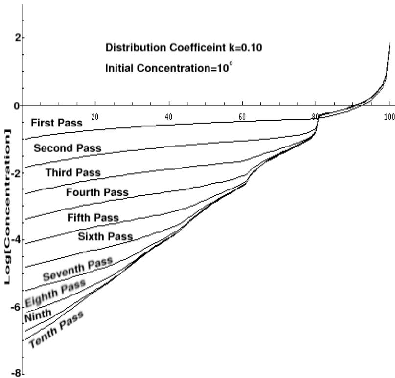
Fig. 2—Concentration profiles in a zone melted rod.
