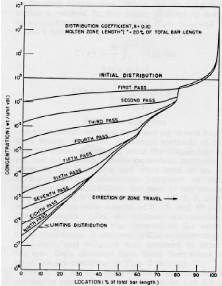
Fig. 2—Concentration profiles in a zone melted rod.
